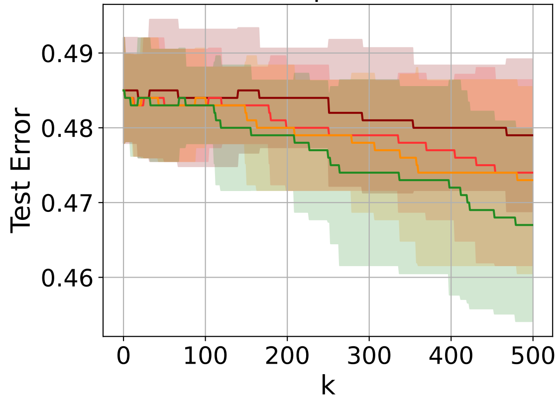
N = 5 particles
