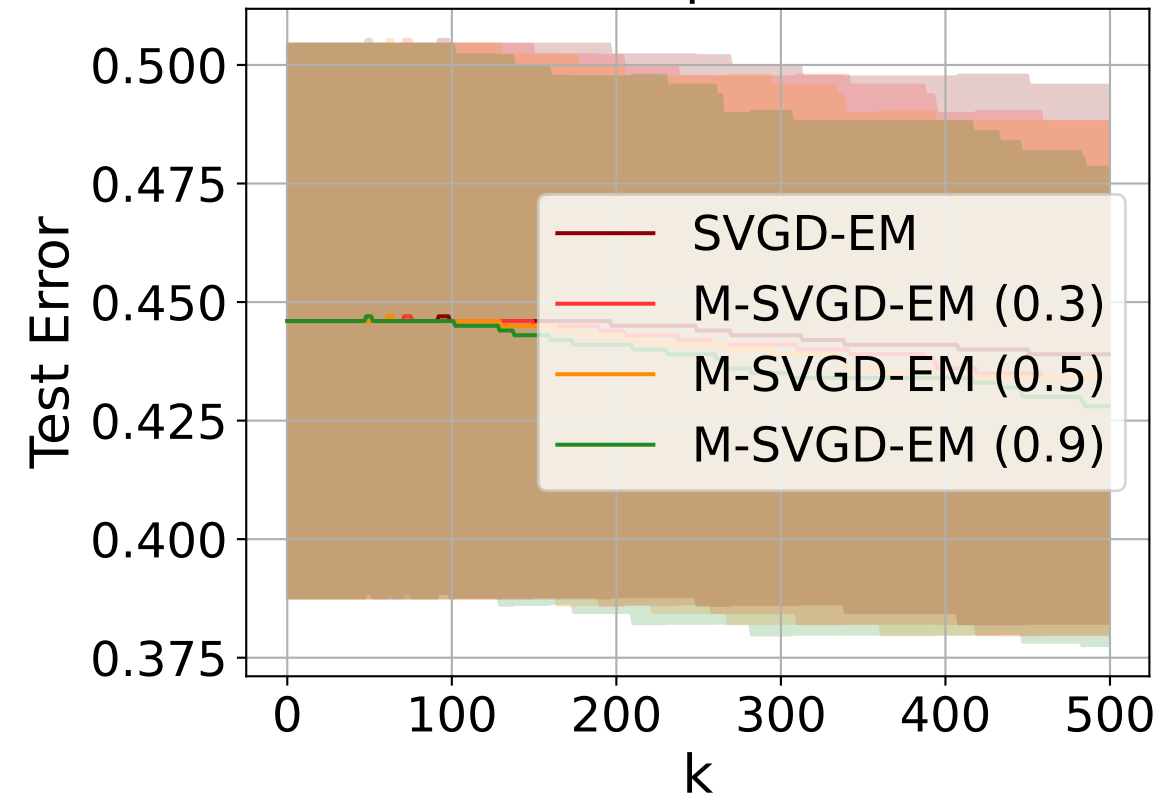
N = 20 particles
