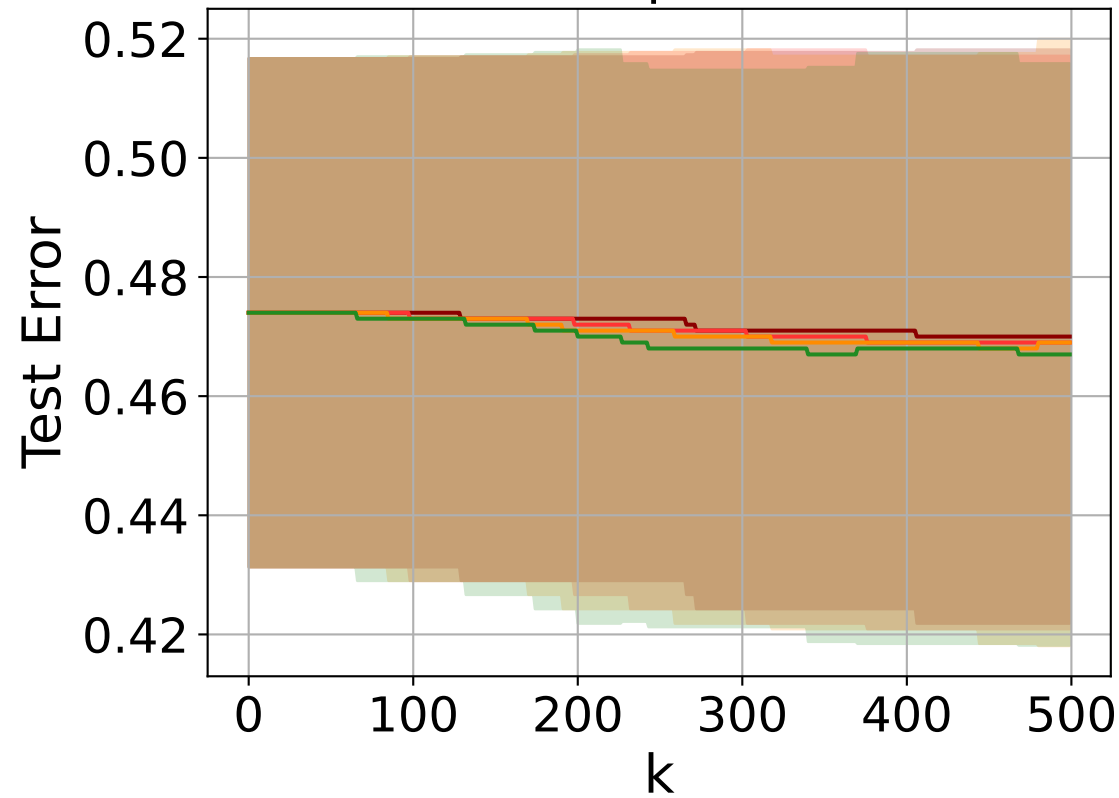
N = 10 particles
